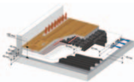
Construction version 3
